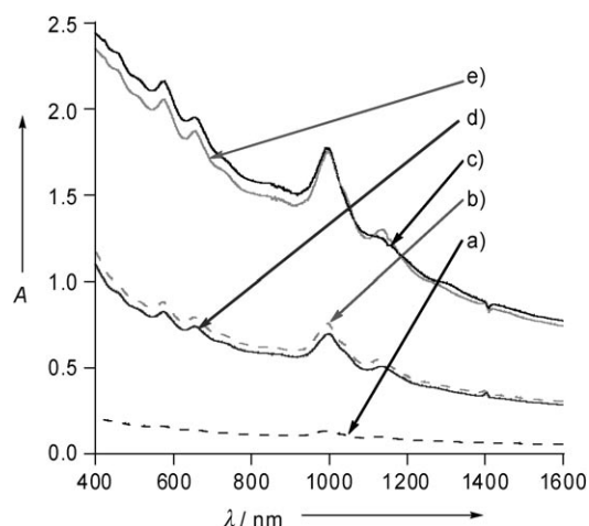
Figure 2. Vis-NIR absorption spectra of SWNTs in chloroform after HSVM in the presence of: a) 1 , b) [\text{Cu}^{\text{II}}(\textbf{1})_2] ( [\text{Cu}^{\text{II}}]/[\textbf{1}]=1:4 ), c) [\text{Cu}^{\text{II}}(\textbf{1})_2] ( [\text{Cu}^{\text{II}}]/[\textbf{1}]=1:2 ), d) [\text{Cu}^{\text{II}}(\textbf{1})_2] + AsA, and e) [\text{Cu}^{\text{II}}(\textbf{1})_2] + AsA + bubbling air at 25 °C ( [\textbf{1}]=0.67 mM, 1 cm cell).
